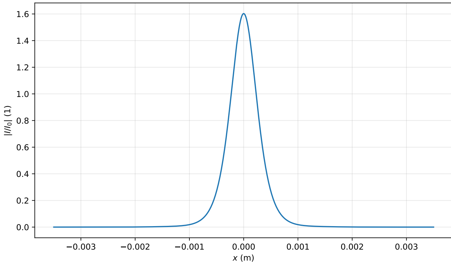
Intensity profile I(x, y = 0, z = 2.707m)/I_0 , P_{in}=0.9P_{cr} , artificial time
